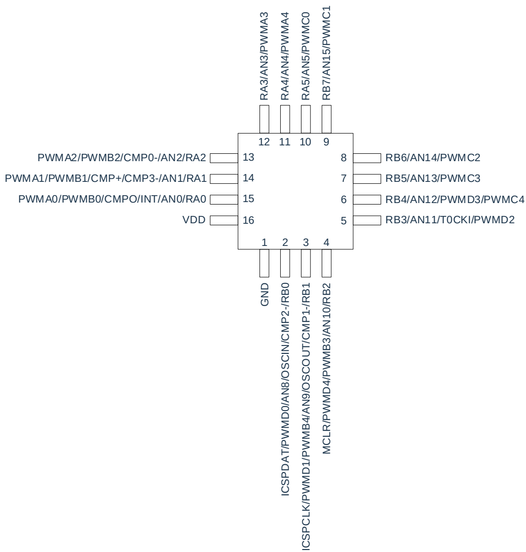
SC8F072AD616NPR
