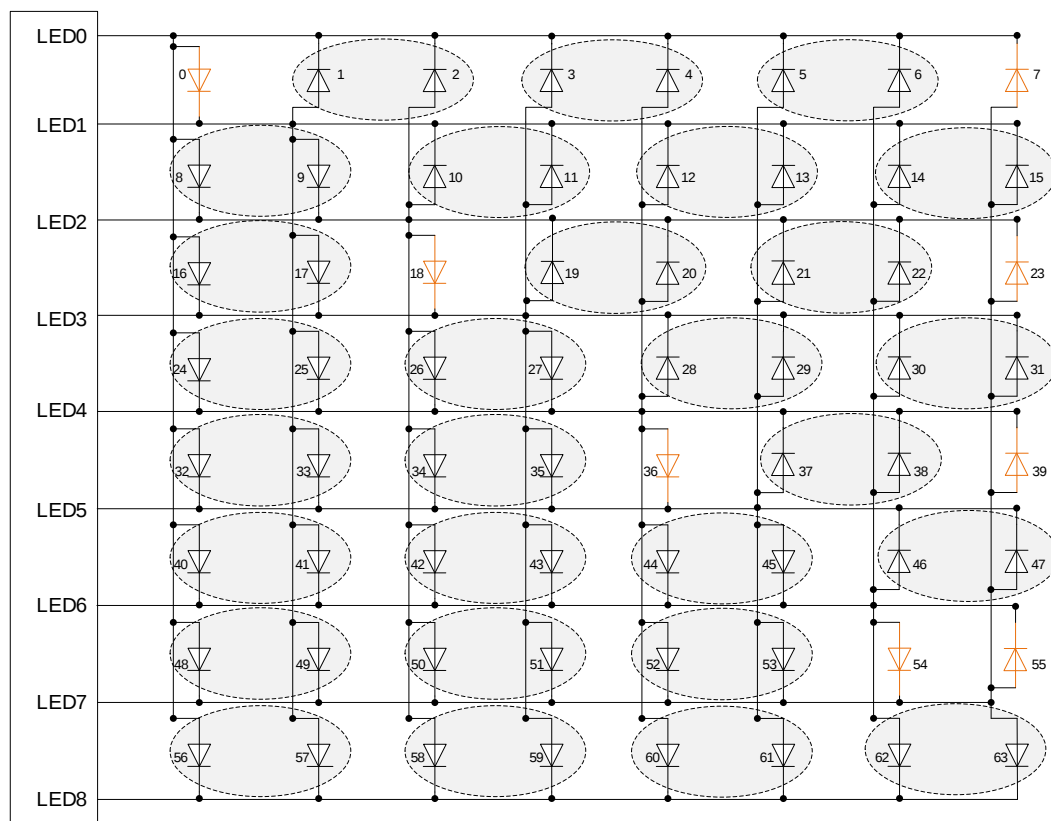
LED 8*8点阵图
