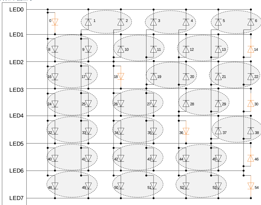
LED 7*7点阵图
