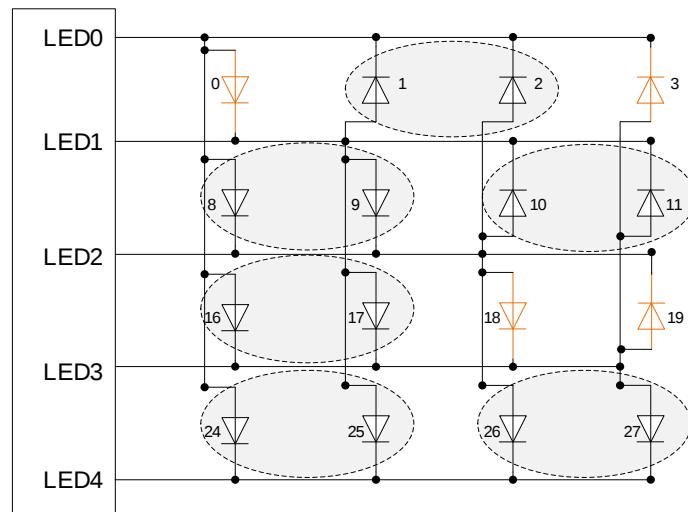
LED 4*4 点阵图
