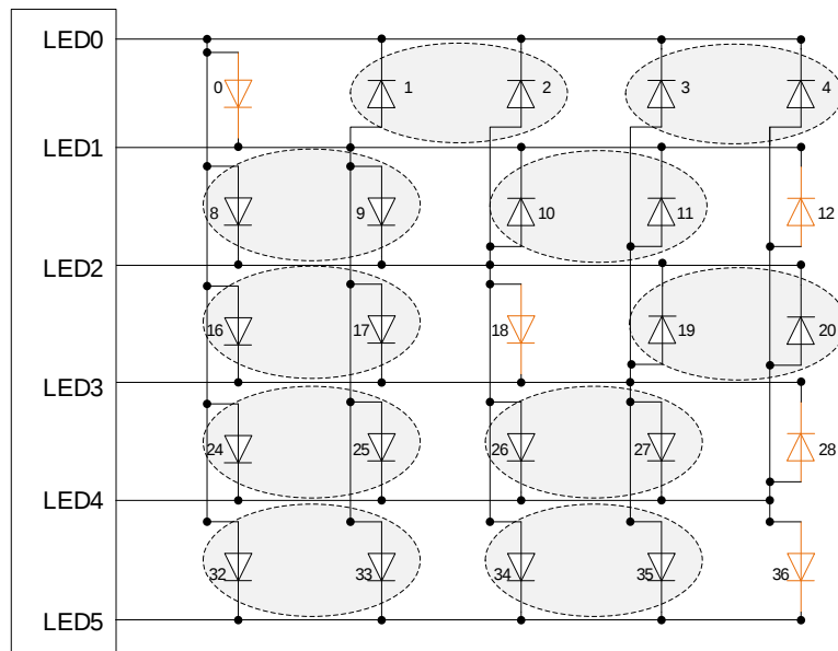
LED 5*5点阵图
