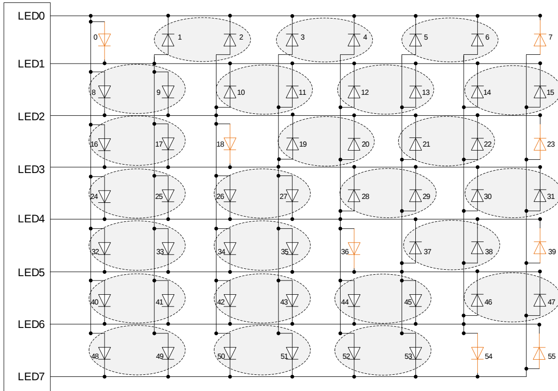
LED 7*8点阵图
