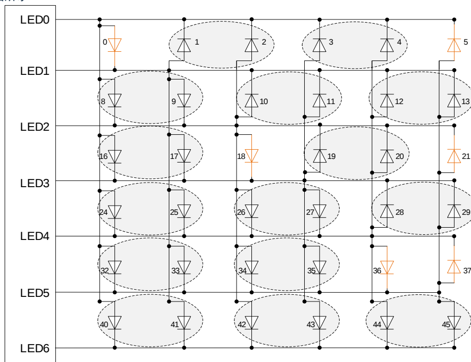
LED 6*6点阵图
