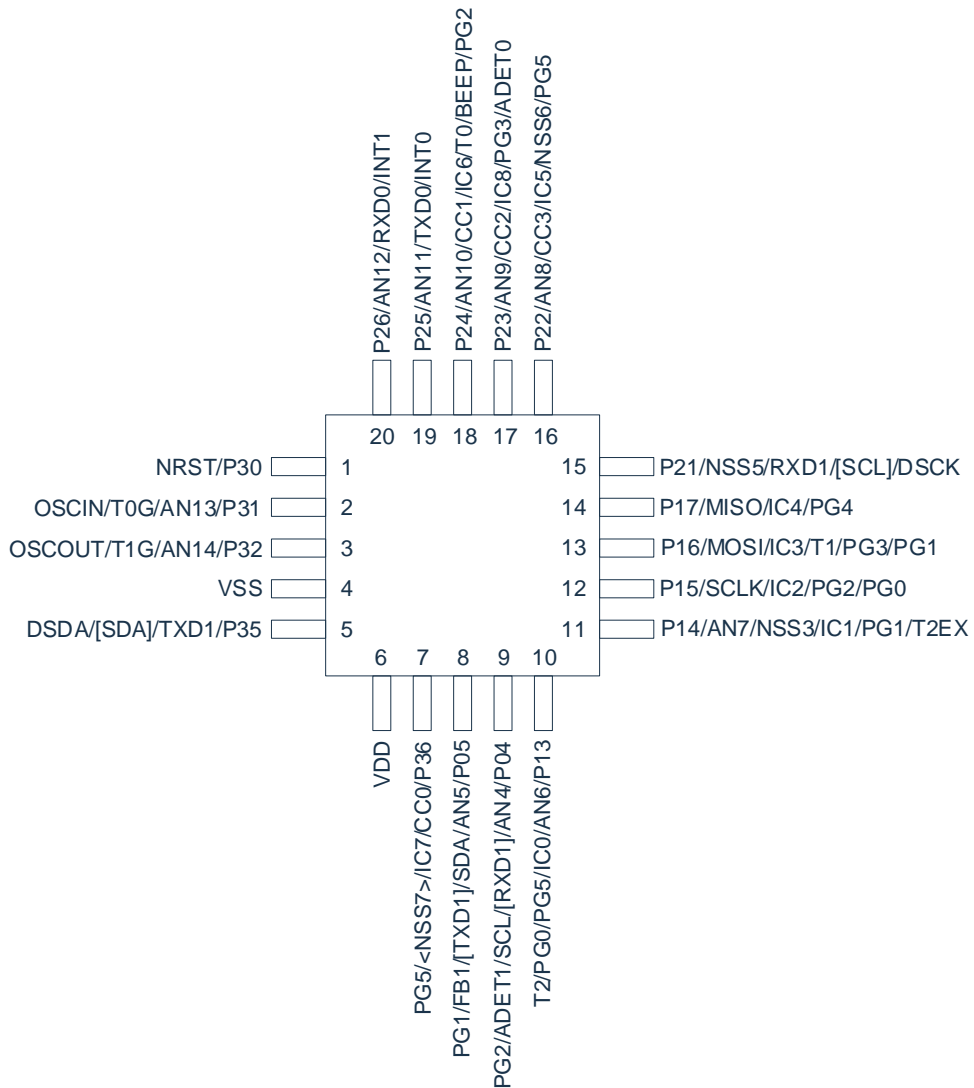
CMS8S5880-QFN20
