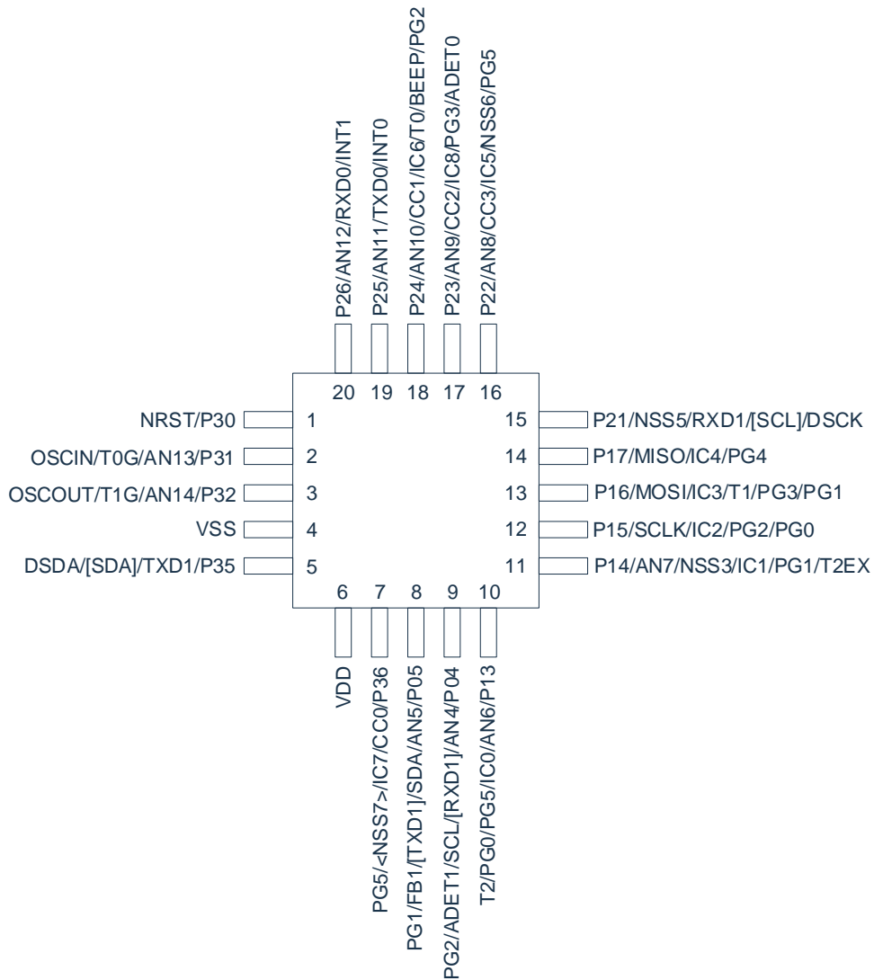
CMS8S5880-QFN20
