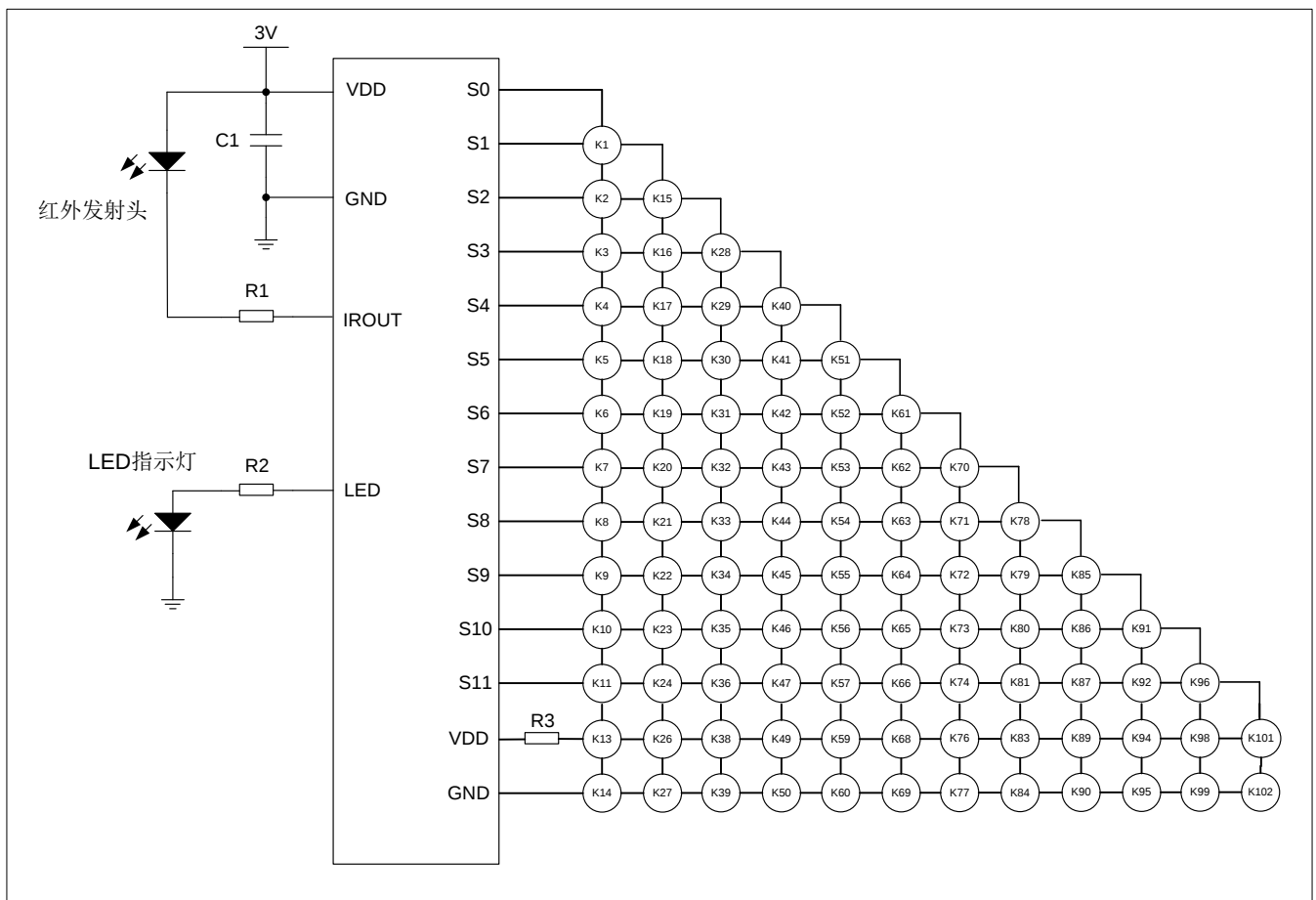
图 2-6: 16PIN 带 LED 输出电路图
