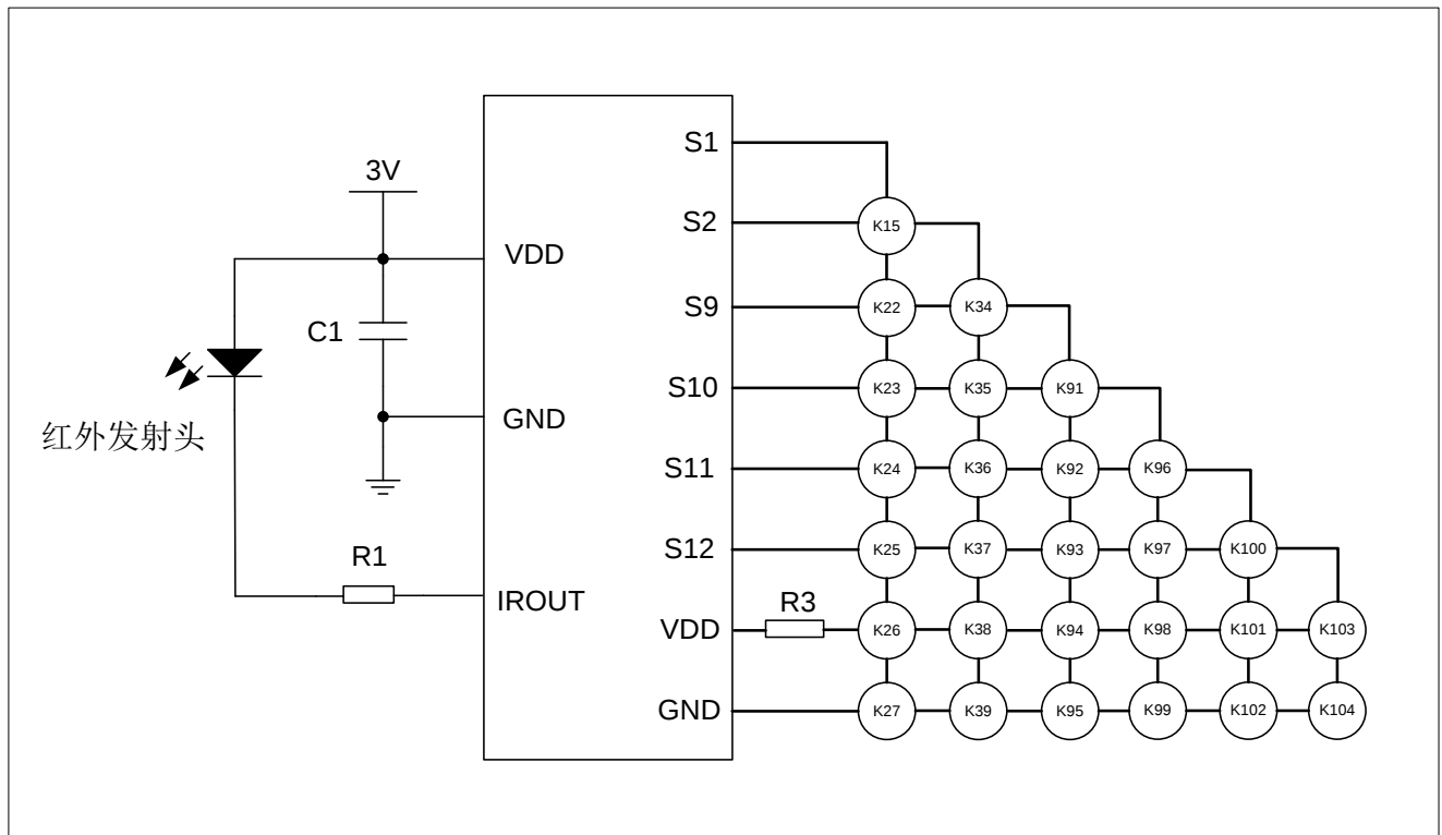
图 2-3: 9PIN 不带 LED 输出电路图
