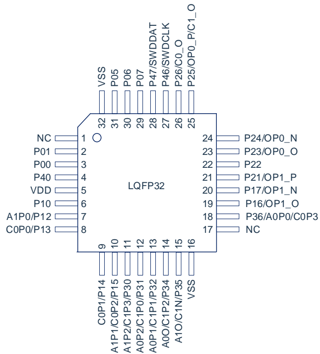
CMS32F033LQ32
