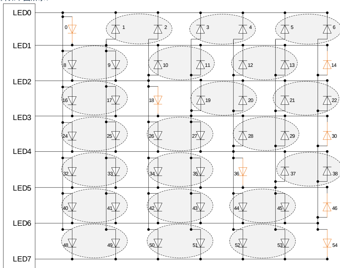
LED 7*7点阵图
