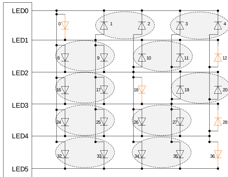
LED 5*5点阵图
