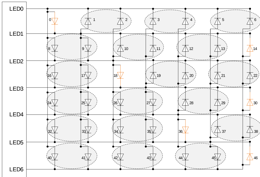
LED 6*7点阵图
