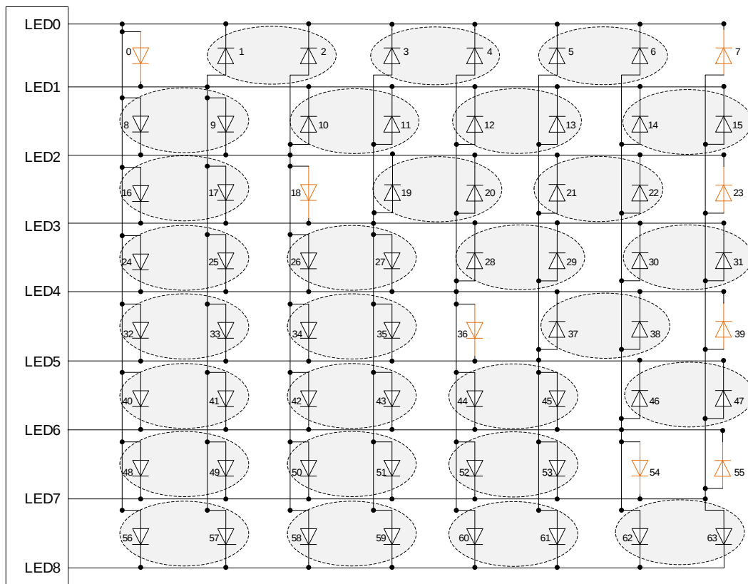
LED 8*8点阵图
