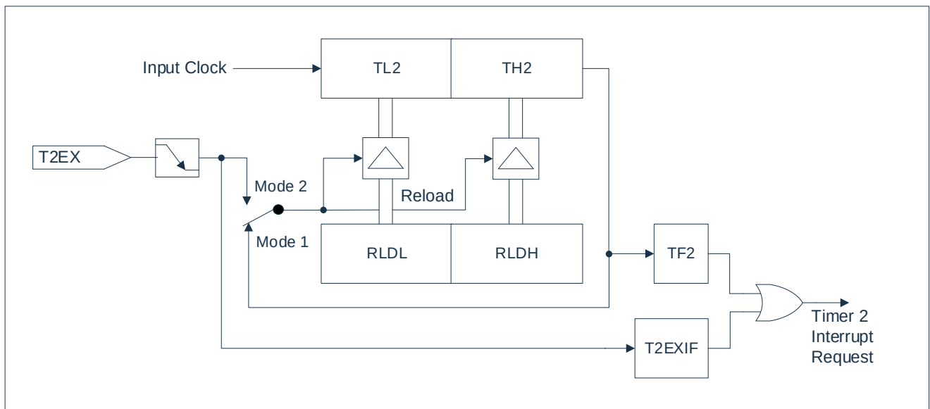
Figure 10-2: Timer2 reload mode block diagram
