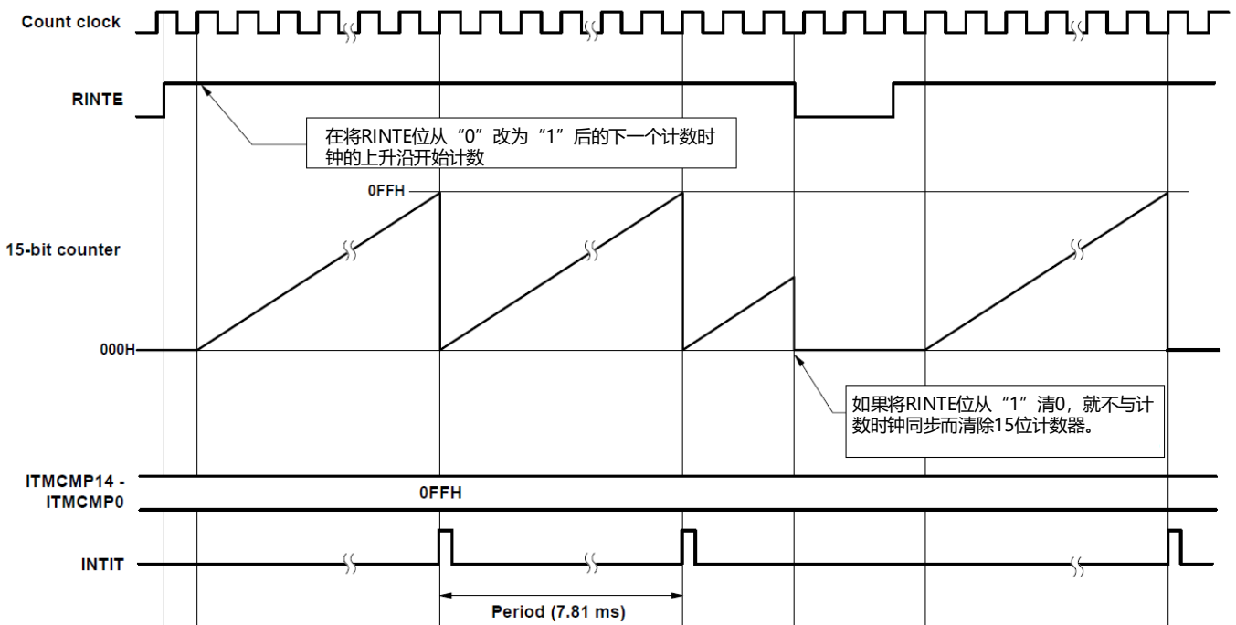
图8-5 15位间隔定时器的运行时序 (ITCMP14~ITCMP0=0FFH, 计数时钟: f_{SUB}=32.768\text{kHz} )
